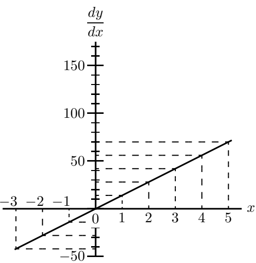
FIG. 6a.—Graph of \frac{dy}{dx} = 14x .
