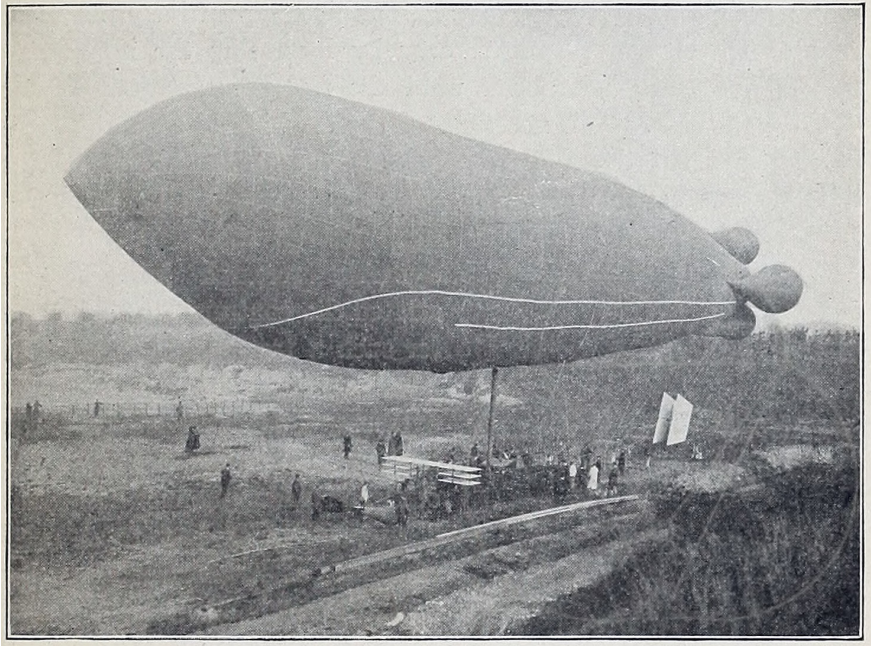
Fig. 13. Clement-Bayard I
